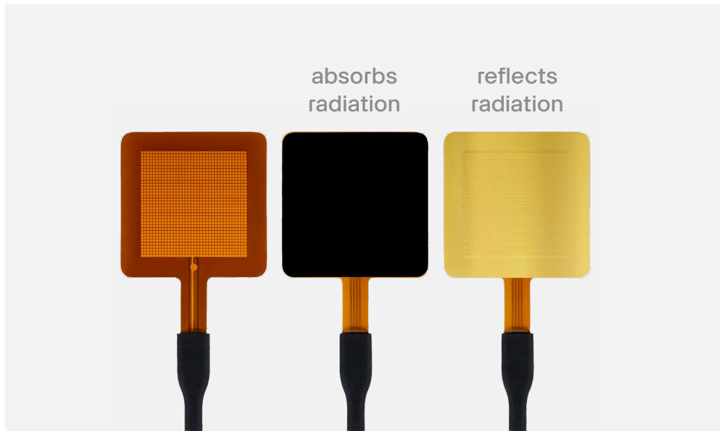
Figure 0.3 FHF05-50X50 with BLK-50X50 and GLD-50X50 stickers.
