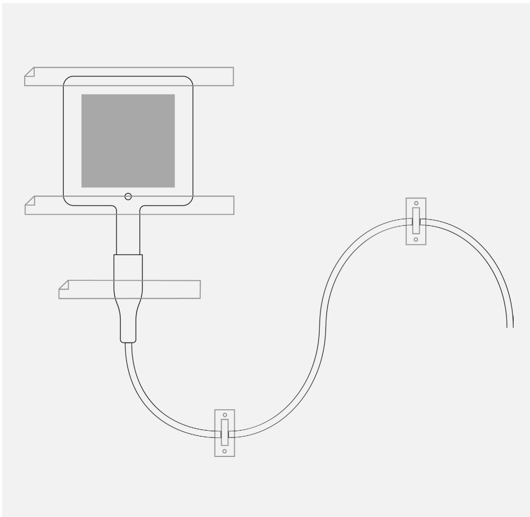
Figure 5.21 Installation of model FHF05-50X50 using tape to fix the sensor and the connection block. Extra strain relief on the cable is provided using cable tie mounts equipped with double-sided tape as an adhesive. As indicated in Table 5.11, tapes used for mounting the sensor are preferably taped over the passive guard area and not on the sensing area (the latter indicated by grey shading in Figure 5.1.1). Please note the dot is visible in this image; this indicates that we are viewing the frontside and that the other side, the backside, is attached to the object on which the sensor is mounted, as in Figure 2.2.
