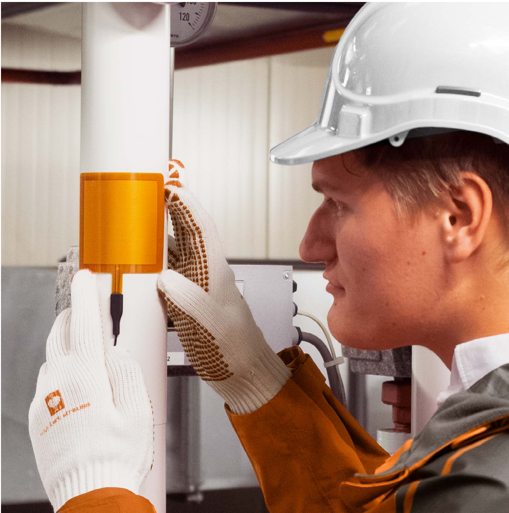
Figure 4.11 Example of model FHF05-85X85 foil heat flux sensor being installed for measurement on an industrial pipe. The sensor is mounted on a well-prepared curved surface.
