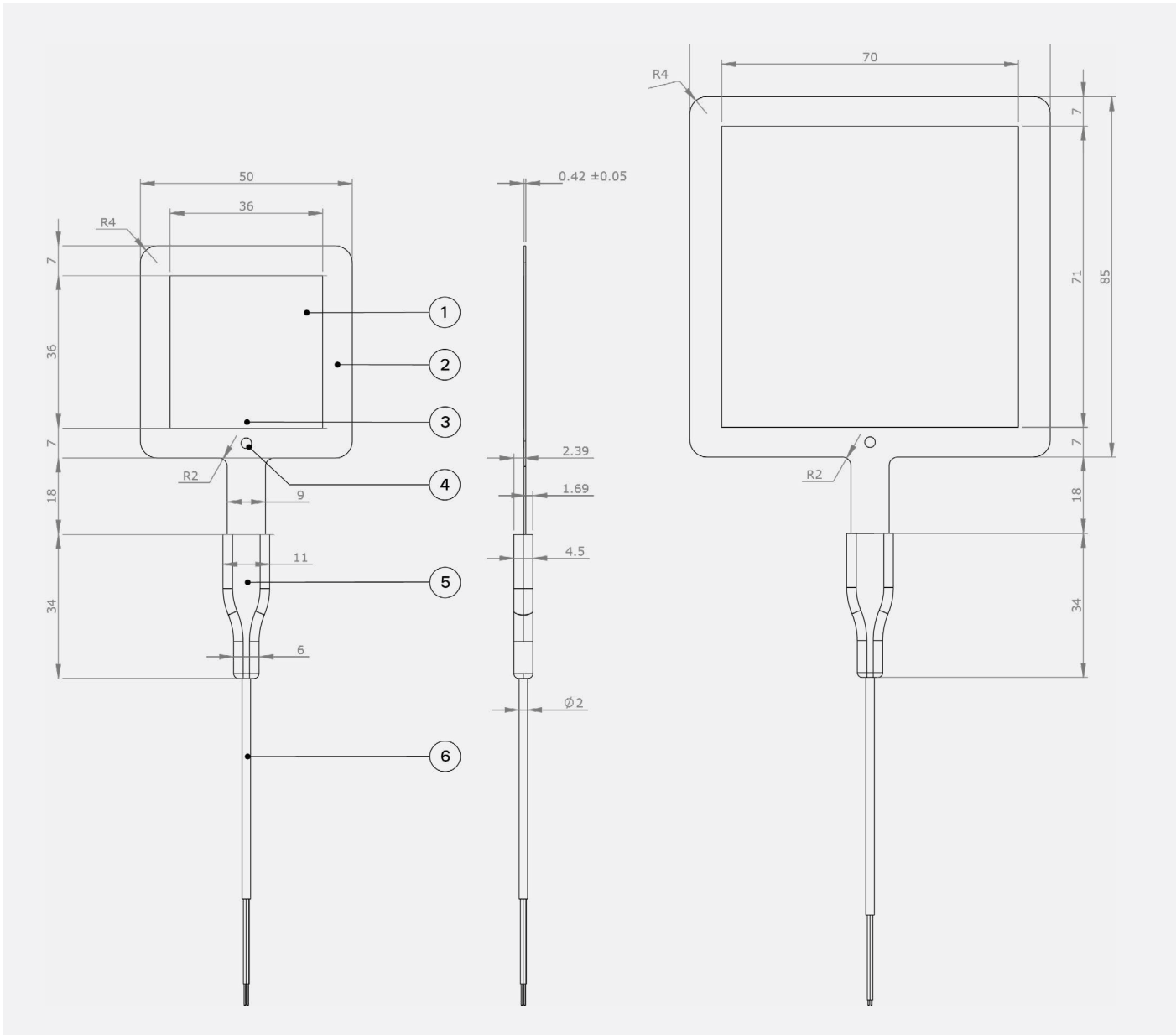
Figure 3.2.2 Models FHF05-50X50, -85X85; with dimensions in \times 10^{-3} m.
