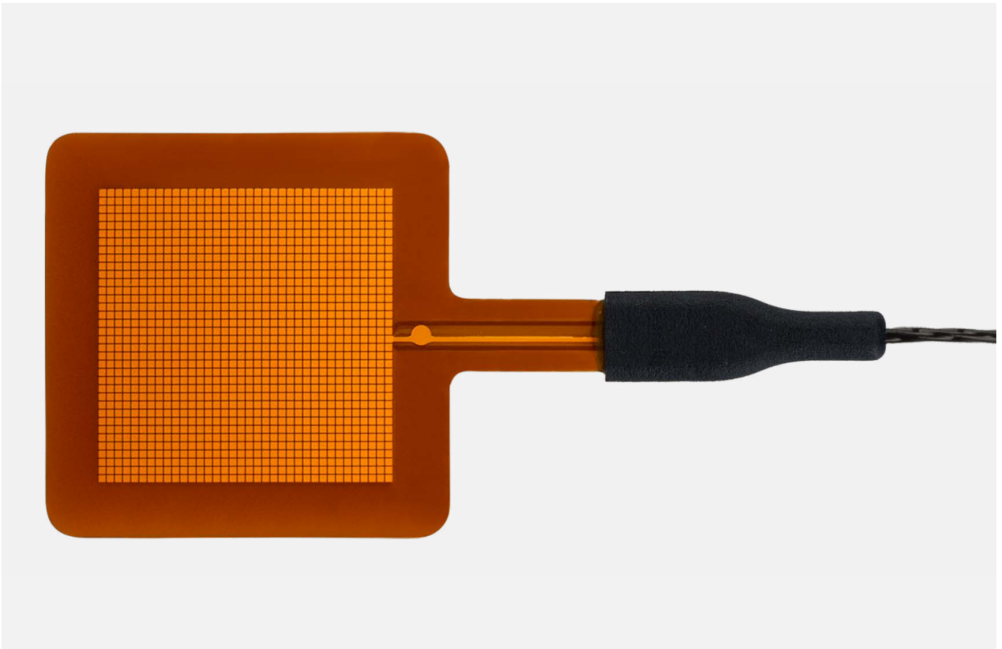
Figure 0.1 FHF05-50X50 foil heat flux sensor with thermal spreaders: thin, flexible, and versatile.
