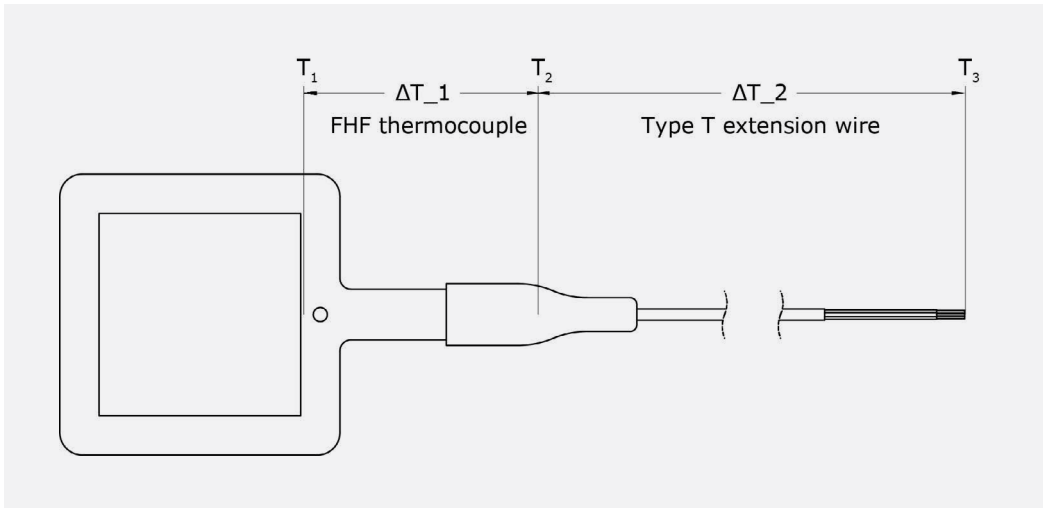
Figure 7.8.1 Model FHF05-50x50 with its thermocouple junctions. To minimize temperature measurement uncertainty, please make sure that \Delta T_1 is close to zero.
