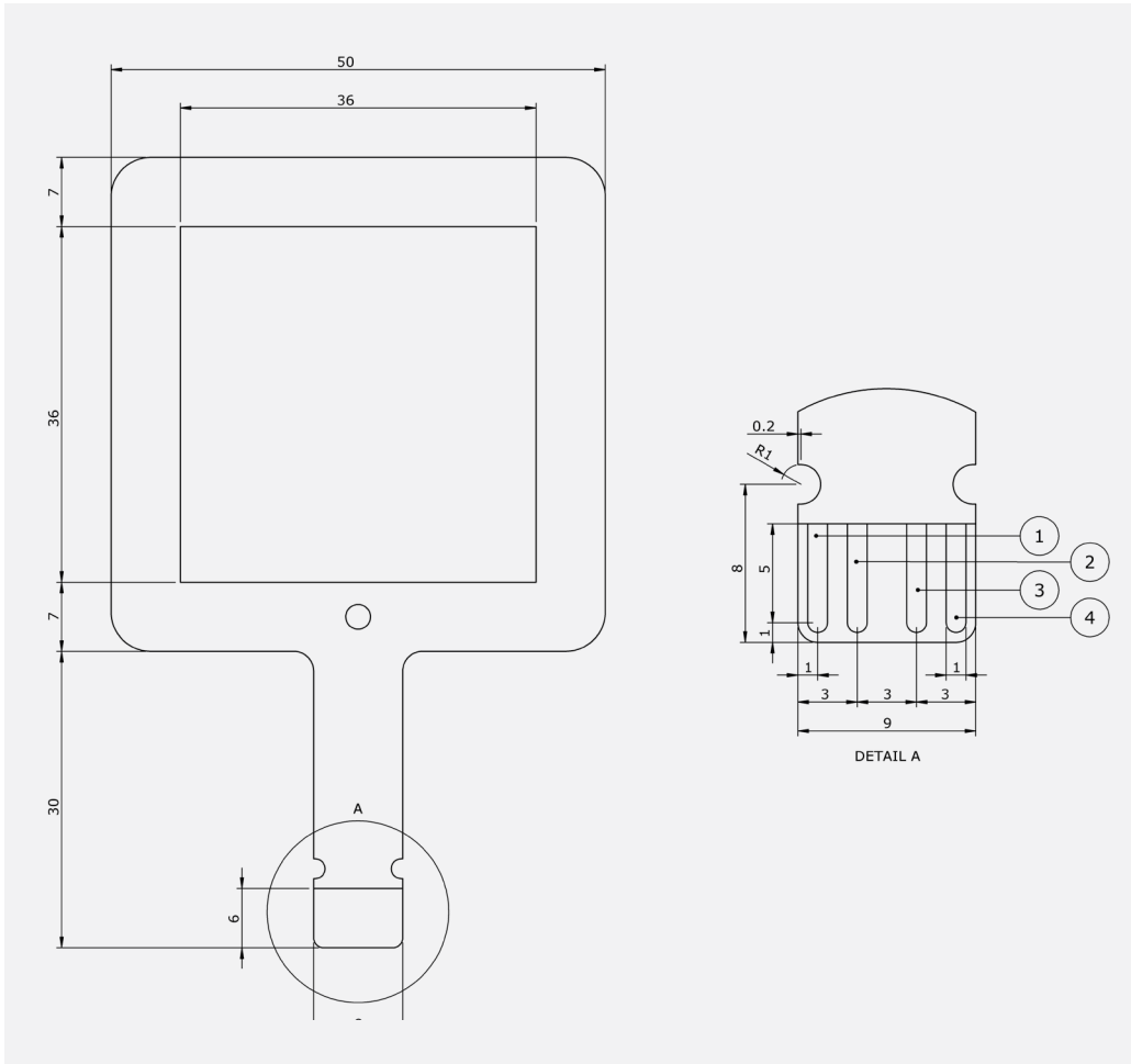
Figure 7.2.1 FHF05-50X50 sensor foil; detail A is the same for all FHF's; dimensions in \times 10^{-3} m. The dimensions of the tab are identical for all FHF sensor models.
