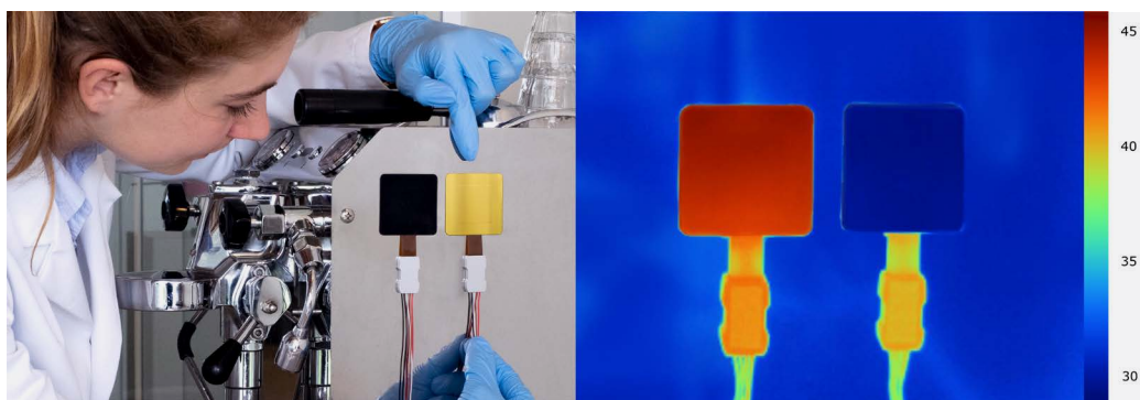
Figure 2.21 Application of a BLK black sticker and a GLD gold sticker on FHF models for measuring radiative and convective heat flux on an espresso machine. The machine has a polished metal surface of about 45 °C. The IR image on the right shows that the black sticker on the left, as well as the sensor wires and connector blocks, emit radiation. They appear in red on the image. The gold sticker and the metal surface have lower emission and appear as “bluish” in the image. Mounted on the same surface, the BLK and GLD stickers have the same temperature. The measurement with the sensor with the GLD sticker is most representative of the heat flux at the polished metal surface, while the sensor with the BLK sticker overestimates the heat flux.
