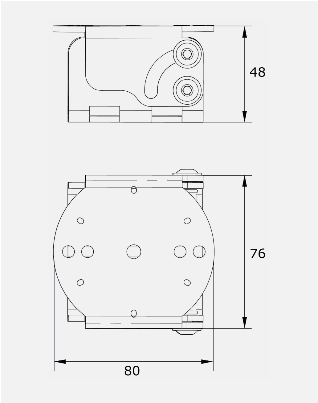
Figure 2.4.1 Dimensions of PMF01 in 10^{-3} m.
