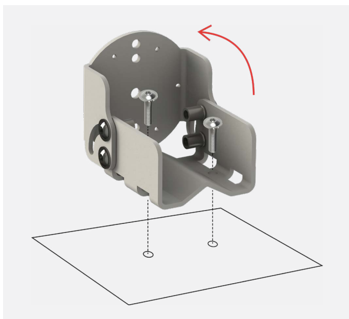
Figure 3.5.2 Installation of PMF01 on a surface, step 2.
