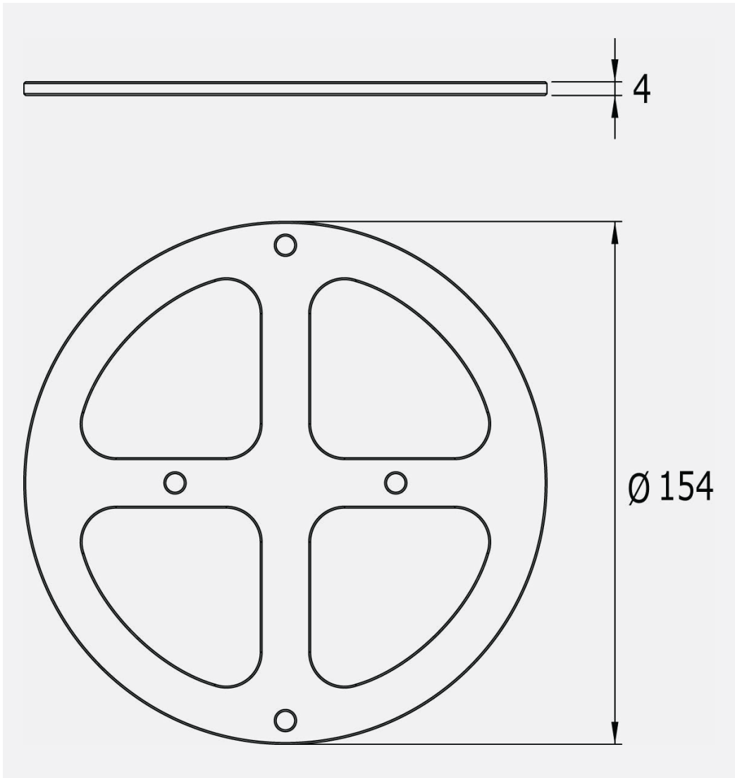
Figure 2.4.2 Dimensions of VMA01 in 10^{-3} m.
