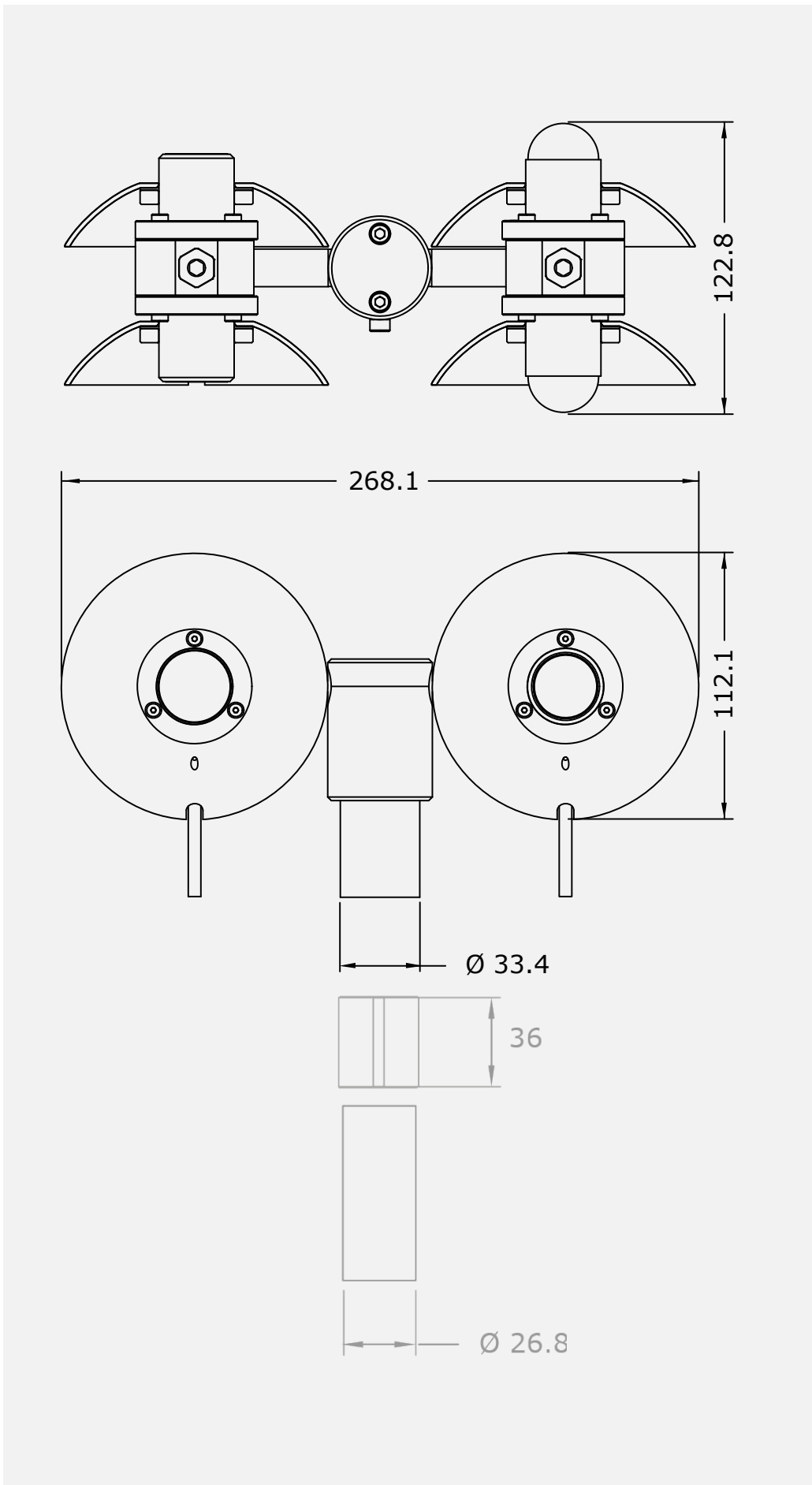
Figure 3.4.1 Dimensions of NR01 in \times 10^{-3} m. NR01 fits a 1 inch NPS tube (recommended outer tube diameter is 33.4 \times 10^{-3} m). Alternatively (displayed in gray), NR01 may be mounted on a \frac{3}{4} inch NPS tube using NR01's shim.
