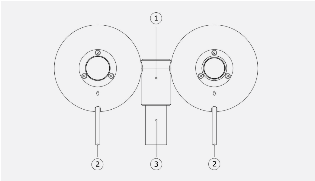
Figure 8.3.3 Top view of RA01 fitting a 1 inch tube: 1. leveling assembly for x- and y-axis 2. cables (cable 1 at the left, at pyranometer side, cable 2 at the right, at pyrgeometer side) 3. 1 inch mounting tube (not included)
