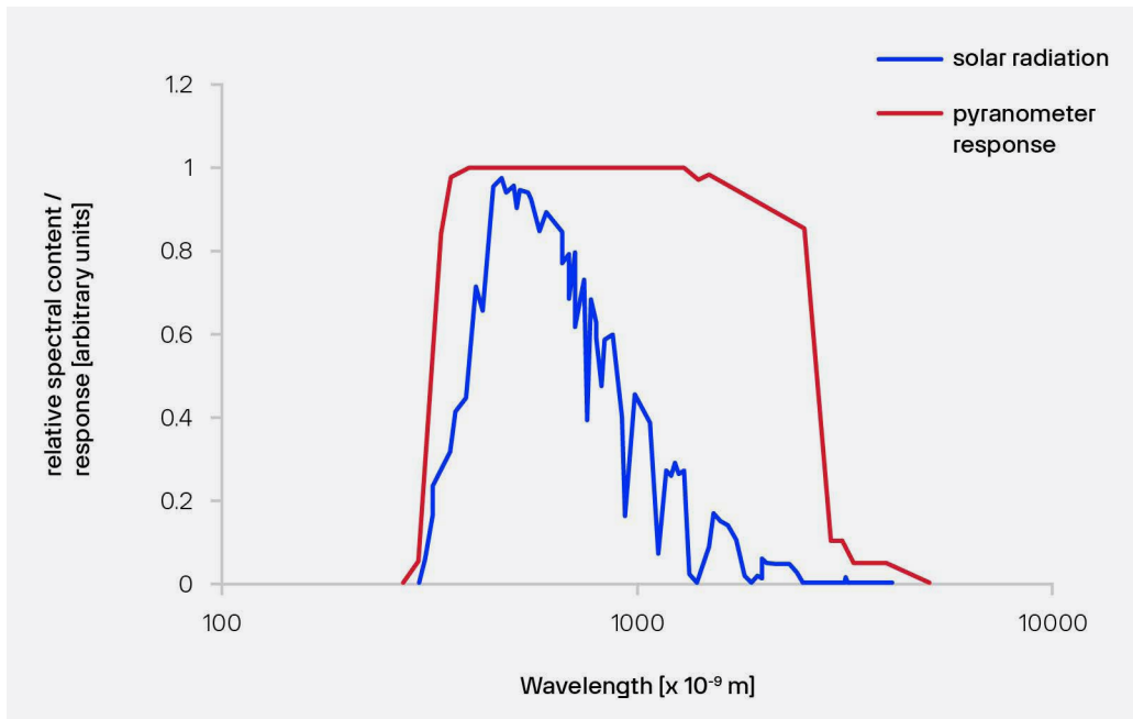
Figure 2.2.1 Spectral response of the pyranometer compared to the solar spectrum. The pyranometer only cuts off a negligible part of the total solar spectrum.
