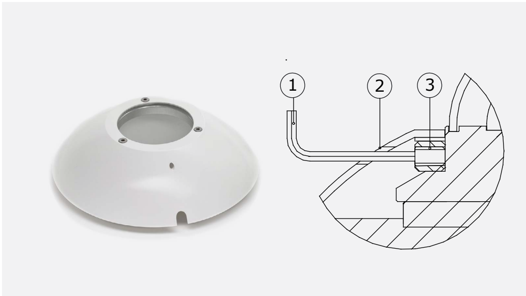
Figure 5.21 SCR01 sun screen and its installation and removal: turn the set screw using the hex key and lift off the sun screen to remove. 1. hex key 2. sun screen 3. set screw
