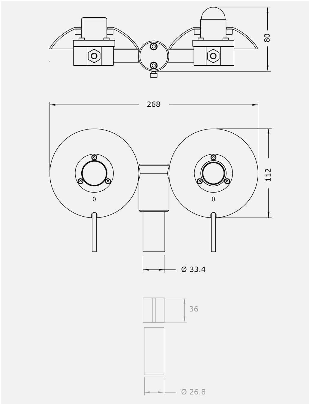
Figure 8.3.1 Dimensions of RA01 in \times 10^{-3} m. RA01 fits a 1 inch NPS tube (recommended outer tube diameter is 33.4 \times 10^{-3} m). Alternatively (displayed in gray), RA01 may be mounted on a \frac{3}{4} inch NPS tube (recommended outer tube diameter is 26.8 \times 10^{-3} m) using RA01's shim.
