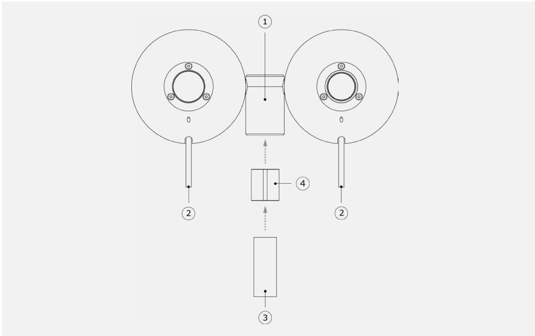
Figure 8.3.4 Top view of RA01 fitting a 3/4 inch NPS tube (alternative mounting method): 1. leveling assembly for x- and y-axis 2. cable (cable 1 at the left, at pyranometer side, cable 2 at the right, at pyrgeometer side) 3. 3/4 inch mounting tube (not included) 4. shim, included with RA01 delivery
