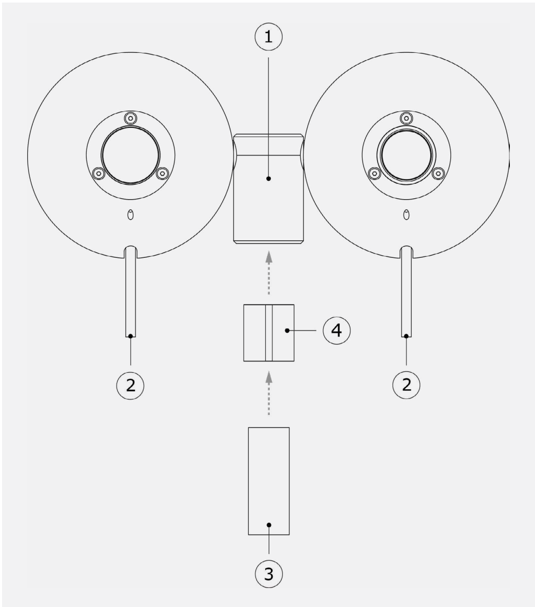
Figure 2.1.3 Top view of NR01 fitting a 3/4 inch NPS tube (alternative mounting method):
