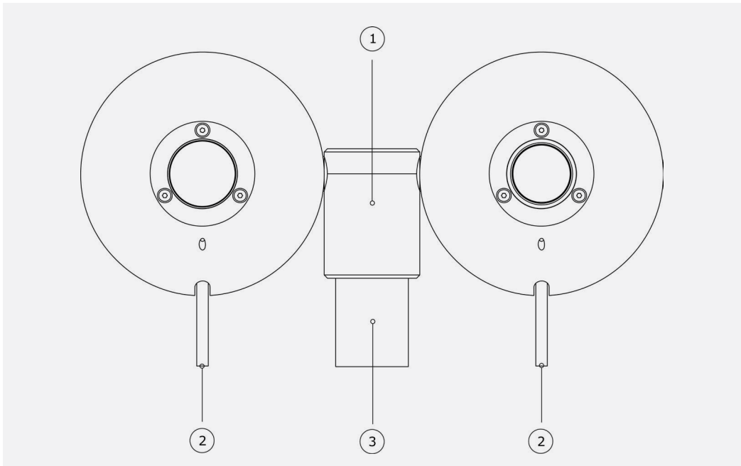
Figure 2.1.2 Top view of NR01 fitting a 1 inch NPS tube:
