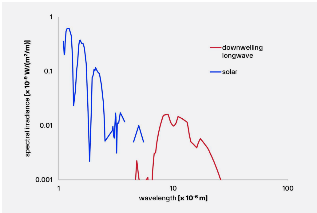
Figure 2.31 Atmospheric radiation as a function of wavelength plotted along two logarithmic axes to highlight the longwave radiation. Longwave radiation is mainly present in the 4 to 50 \times 10^{-6} m range, whereas solar radiation is mainly present in the 0.3 to 3 \times 10^{-6} m range. In practice, the two are measured separately using pyrgeometers and pyranometers.
