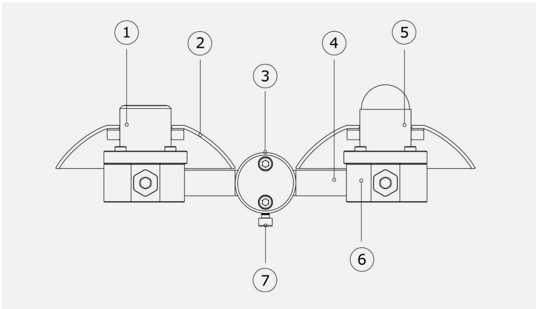
Figure 8.3.2 Overview of RA01: 1. upfacing pyrgeometer 2. sun screens 3,4. leveling assembly for x- and y-axis 5. upfacing pyranometer 6. instrument body 7. leveling assembly for x- and y-axis
