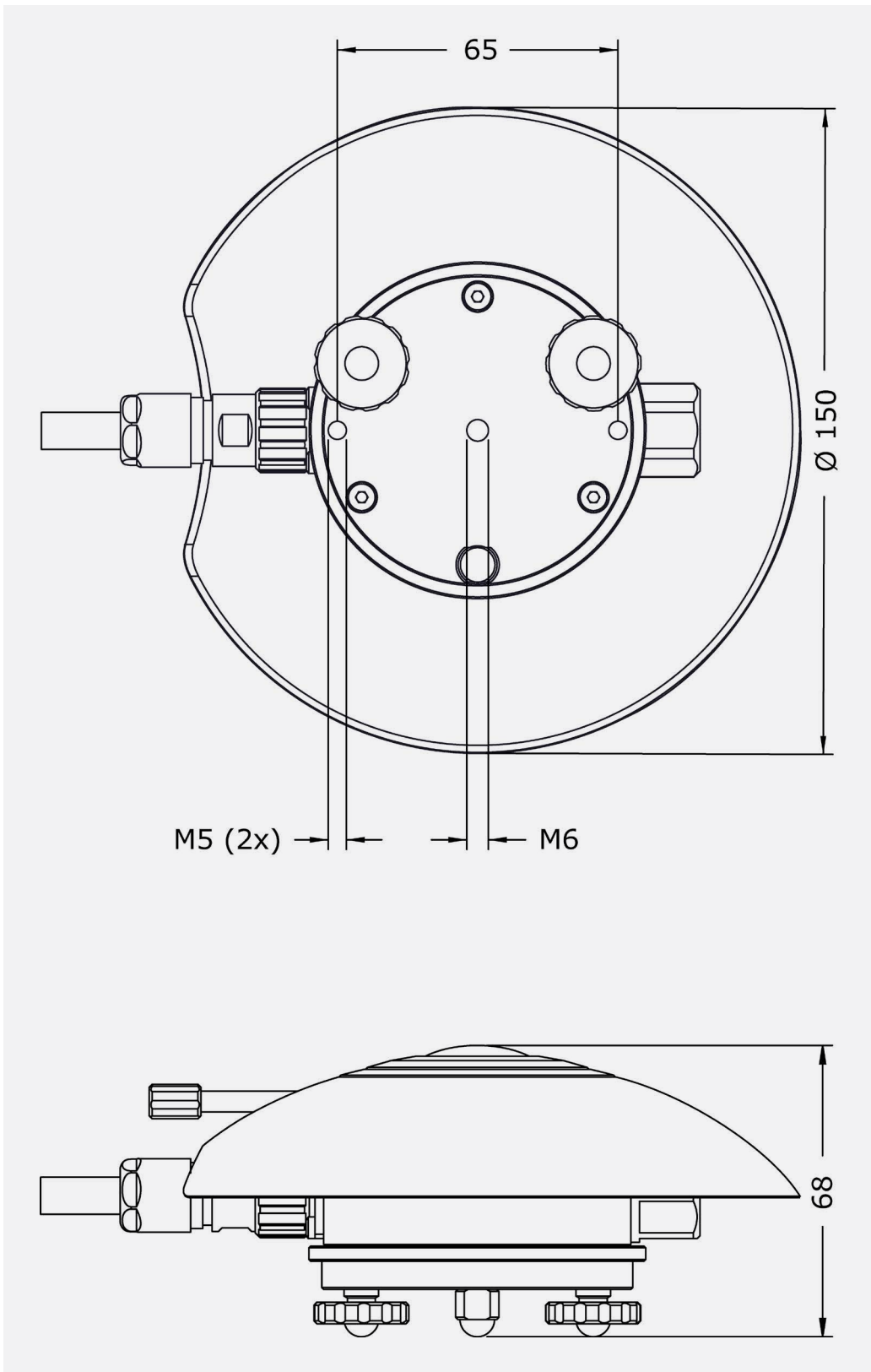
Figure 3.2.1 Dimensions of IR20 and IR20WS in 10^{-3} .
