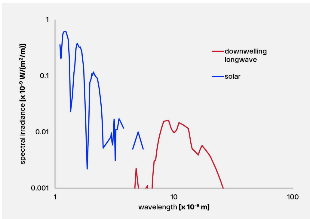
Figure 2.2.1 Atmospheric radiation as a function of wavelength plotted along two logarithmic axes to highlight the longwave radiation. Longwave radiation is mainly present in the 4 to 50 \times 10^{-6} m range, whereas solar radiation is mainly present in the 0.3 to 3 \times 10^{-6} m range. In practice, the two are measured separately using pyrgeometers and pyranometers.
