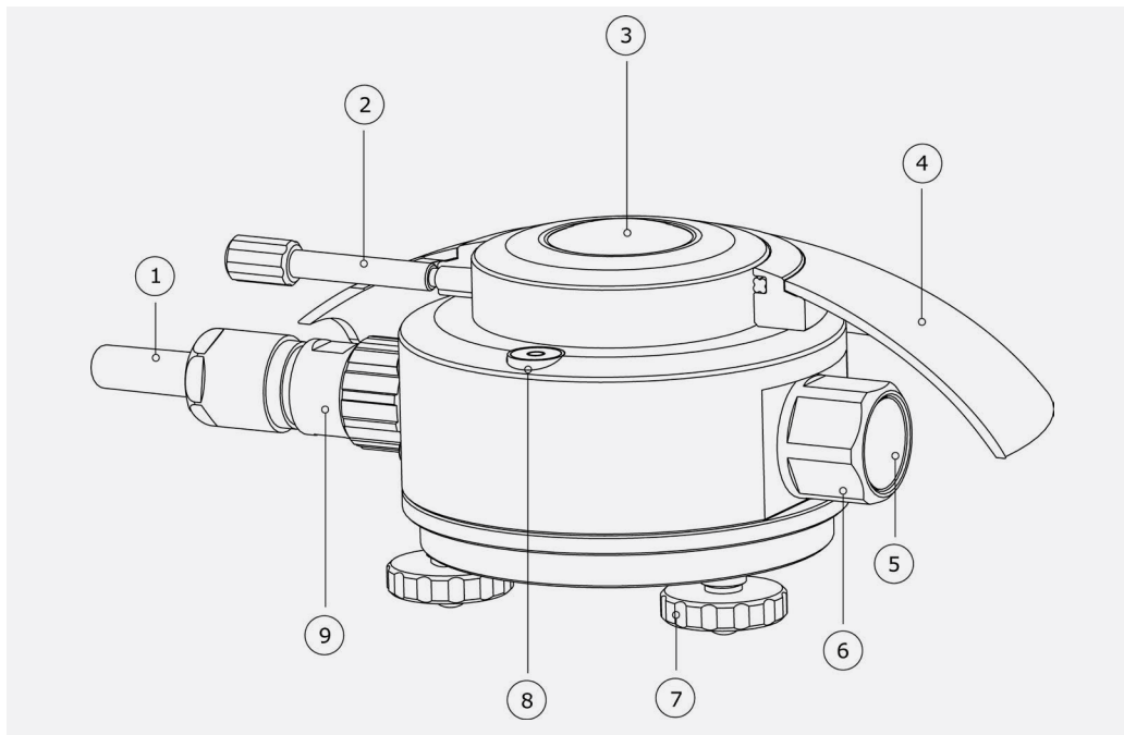
Figure 2.31 Overview of IR20 pyrgeometer:
