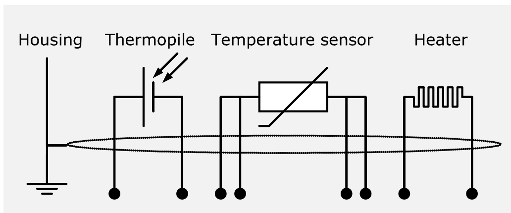
Figure 4.3.1 Electrical diagram of the internal wiring of IR20. The shield is connected to the sensor body.
