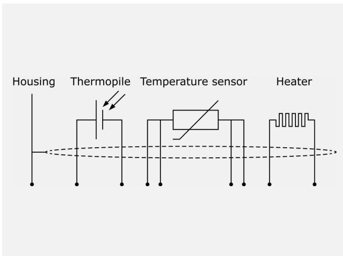
Figure 5.3.2 Electrical diagram of the internal wiring of DR20 / DR15. The shield is connected to the sensor body.
