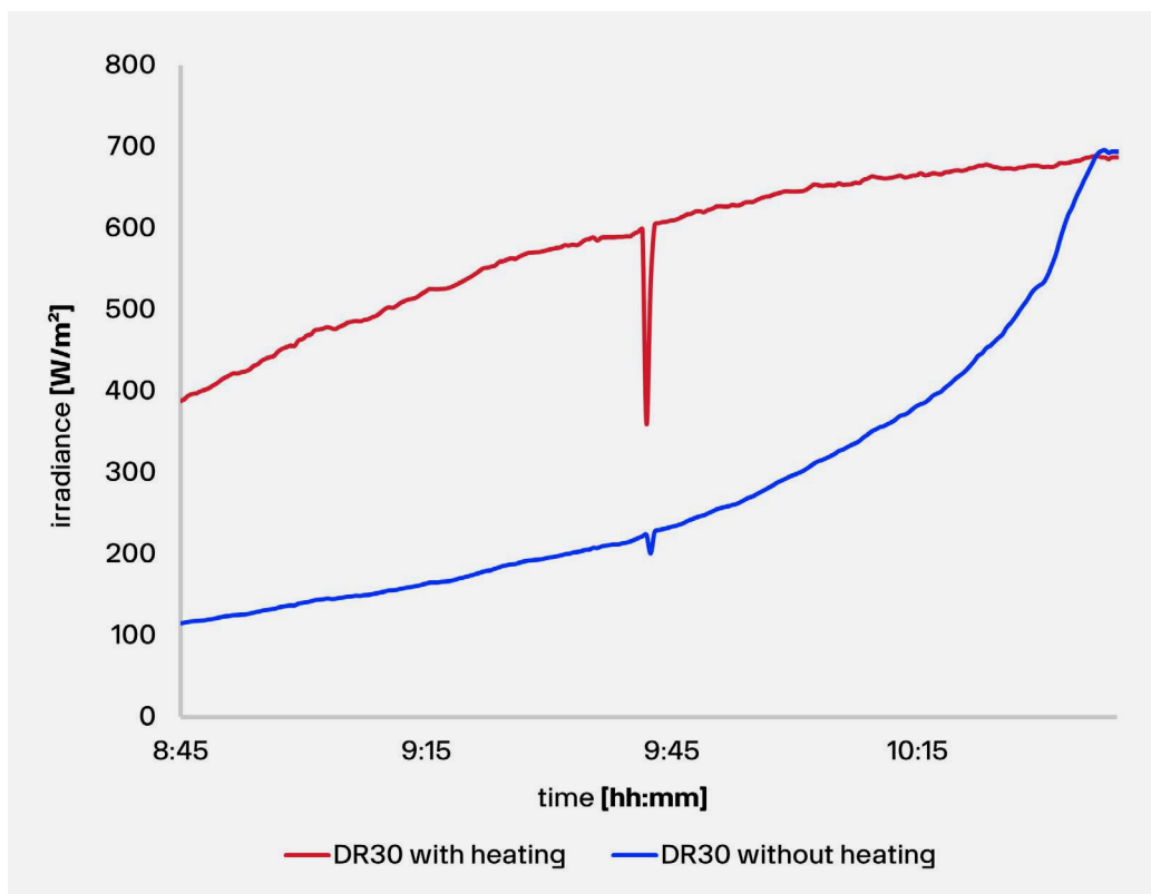
Figure 2.2.2 Comparison of the measured data with and without heating on a typical winter morning, using model DR30 which has the same heating as DR20 and DR15. The unheated DR30 has dew on its front window and strongly underestimates the incoming irradiance. At around 10:30 the dew evaporates. Real measured data from Delft, the Netherlands.
