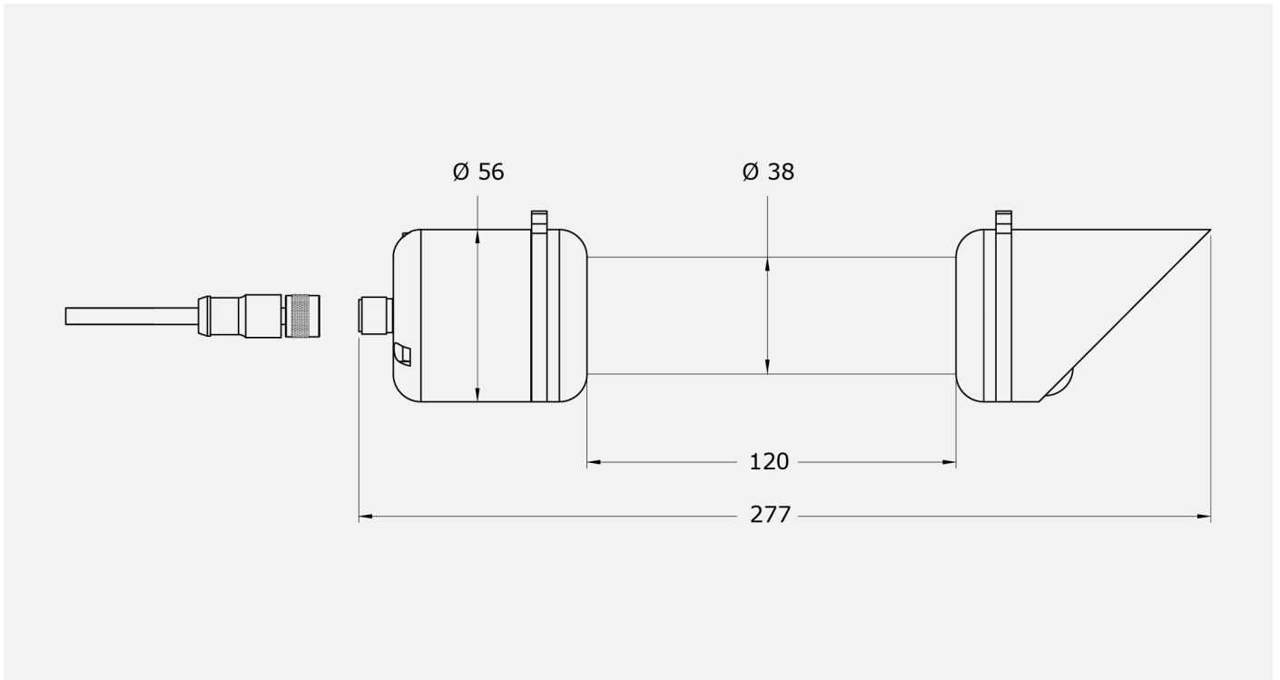
Figure 3.2.1 DR20 / DR15 dimensions in \times 10^{-3} m.
