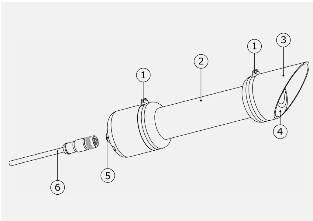
Figure 2.1 Overview of the DR20 / DR15 pyrhelimeter. Versions DR20-A1 and DR15-A1 have an identical external housing.
