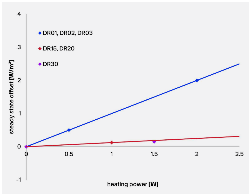
Figure 2.2.1 The offset of the latest models DR20, DR15 (and also the digital DR30) when heating, is much improved relative to the older DR01, DR02 and DR03 models. DR20 and DR15 have a 12 VDC, 1 W heater which produces a negligible offset. The older models had offsets of the order of 1 W/m 2 at the same heating level. In addition, the temperature of the front window of DR20 and DR15 is 4 times higher than that of the older models, at the same heating power.
