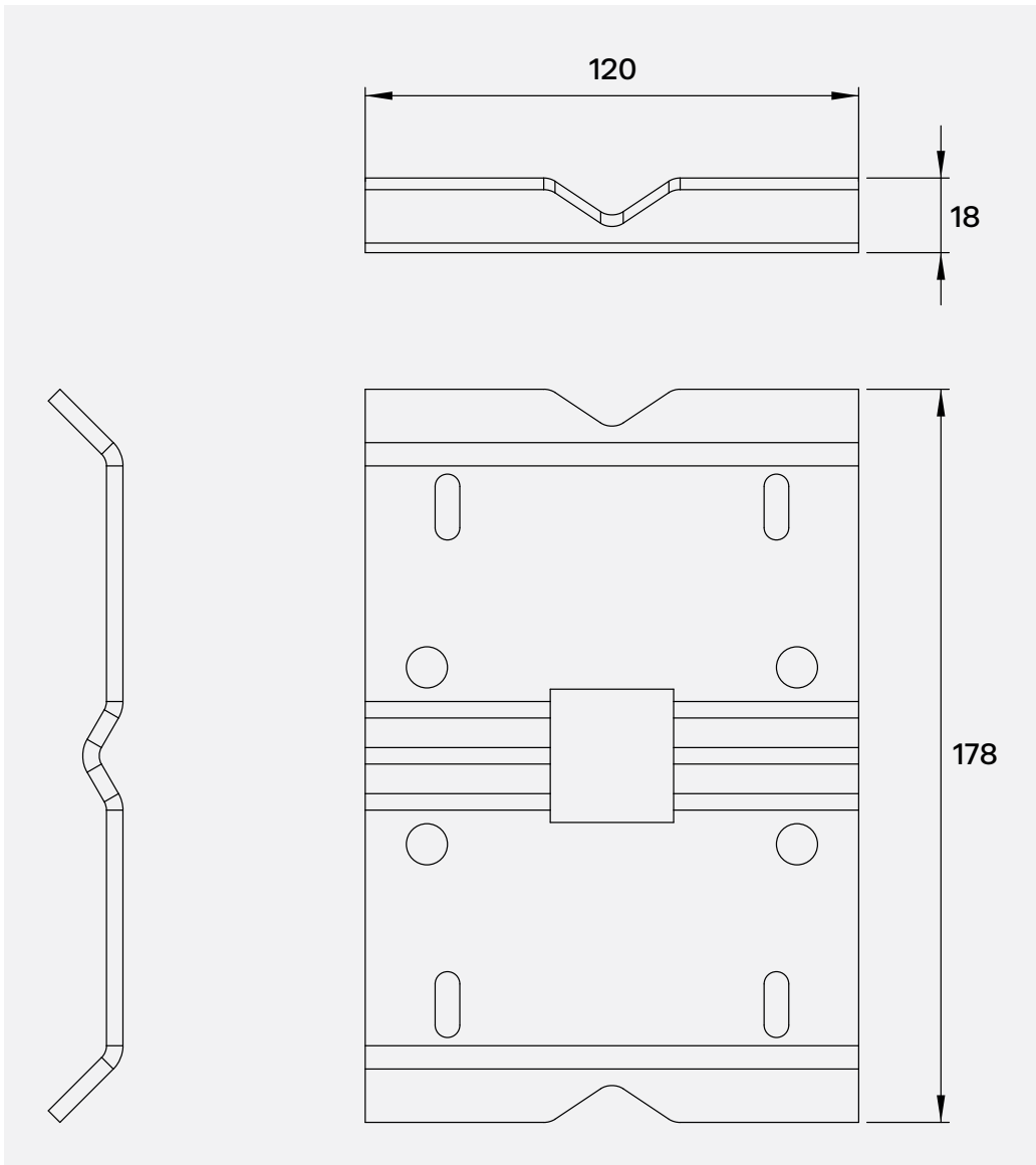
Figure 2.2.1 Dimensions of CMF01 in 10^{-3} .
