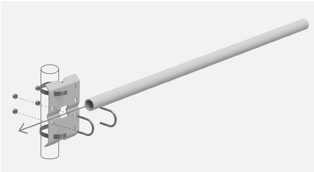
Figure 3.2.2 Step 2: installation of a horizontal crossarm onto CMF01.
