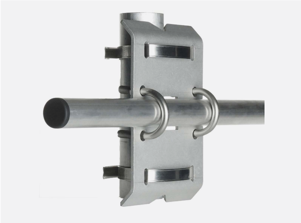
Figure 0.2 CMF01 crossarm mounting fixture, shown with a crossarm mounted on a mast.
