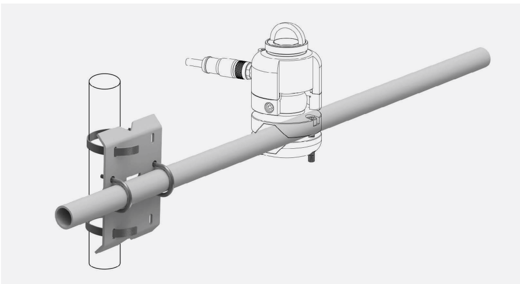
Figure 3.3.3 Step 3: installation of a radiometer on a crossarm, mounted with CMF01 on a mast. Pyranometer model SR05 with tube leveling is shown as an example.
