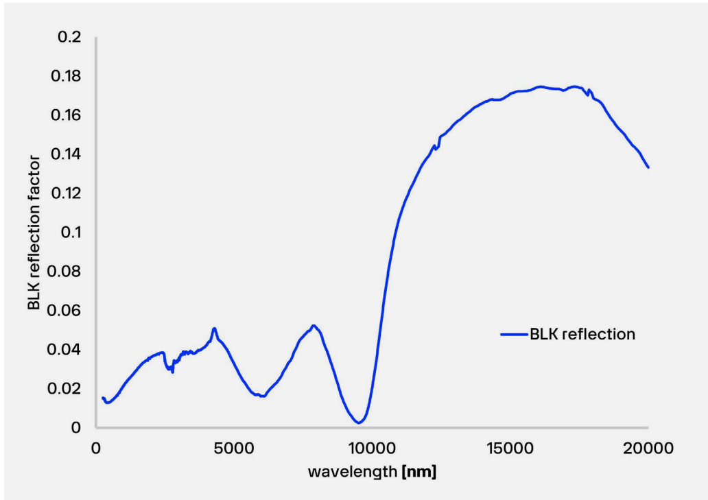
Figure 8.1.1 Reflection factor of BLK sticker as a function of the wavelength of the incoming radiation.
