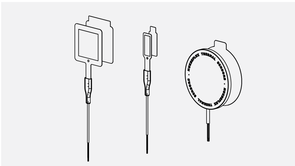
Figure 5.2.2 The dimensions of the BLK – GLD stickers match the dimensions of the corresponding heat flux sensors FHF05 series and HFP01.
