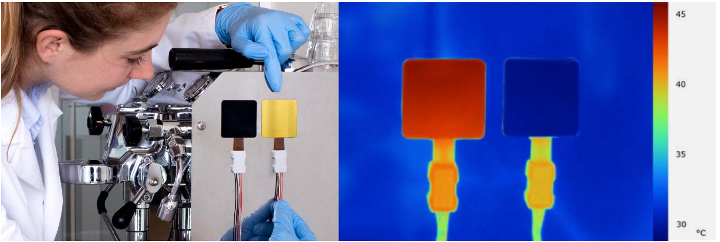
Figure 4.11 Measuring with BLK – GLD stickers; application of a BLK black sticker and a GLD gold sticker on FHF models for measuring radiative and convective heat flux on an espresso machine. The machine has a polished metal surface of about 45 °C. The IR image on the right shows that the black sticker on the left, as well as the sensor wires and connector cable connection blocks, emit radiation. They appear in red on the image. The gold sticker and the metal surface have lower emission and appear as “bluish” on the image. Mounted on the same surface, the BLK and GLD stickers have the same temperature. The measurement with the sensor with the GLD sticker is most representative of the heat flux at the polished metal surface, while the sensor with the BLK sticker overestimates the heat flux. The sensor tabs, cable connection blocks and cable are not connected to the metal plate and have a temperature between that of the metal and ambient air.
