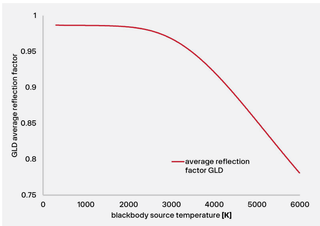
Figure 8.1.4 Average reflection factor of GLD sticker when measuring radiation from blackbody sources of different temperatures.
