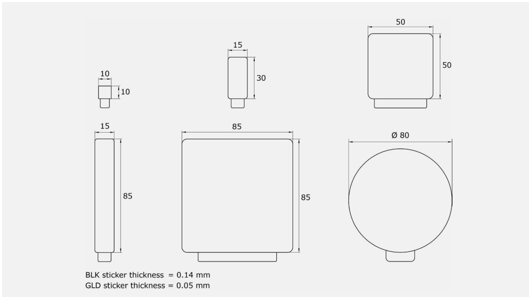
Figure 5.2.1 Dimensions of BLK – GLD stickers; all dimensions in \times 10^{-3} m for both BLK and GLD stickers. Top row from left to right: -10X10, -15X30, -50X50. Bottom row from left to right: -15X85, -85X85 and -80. All BLK stickers have a thickness of 0.14 mm, GLD stickers have a thickness of 0.05 mm.
