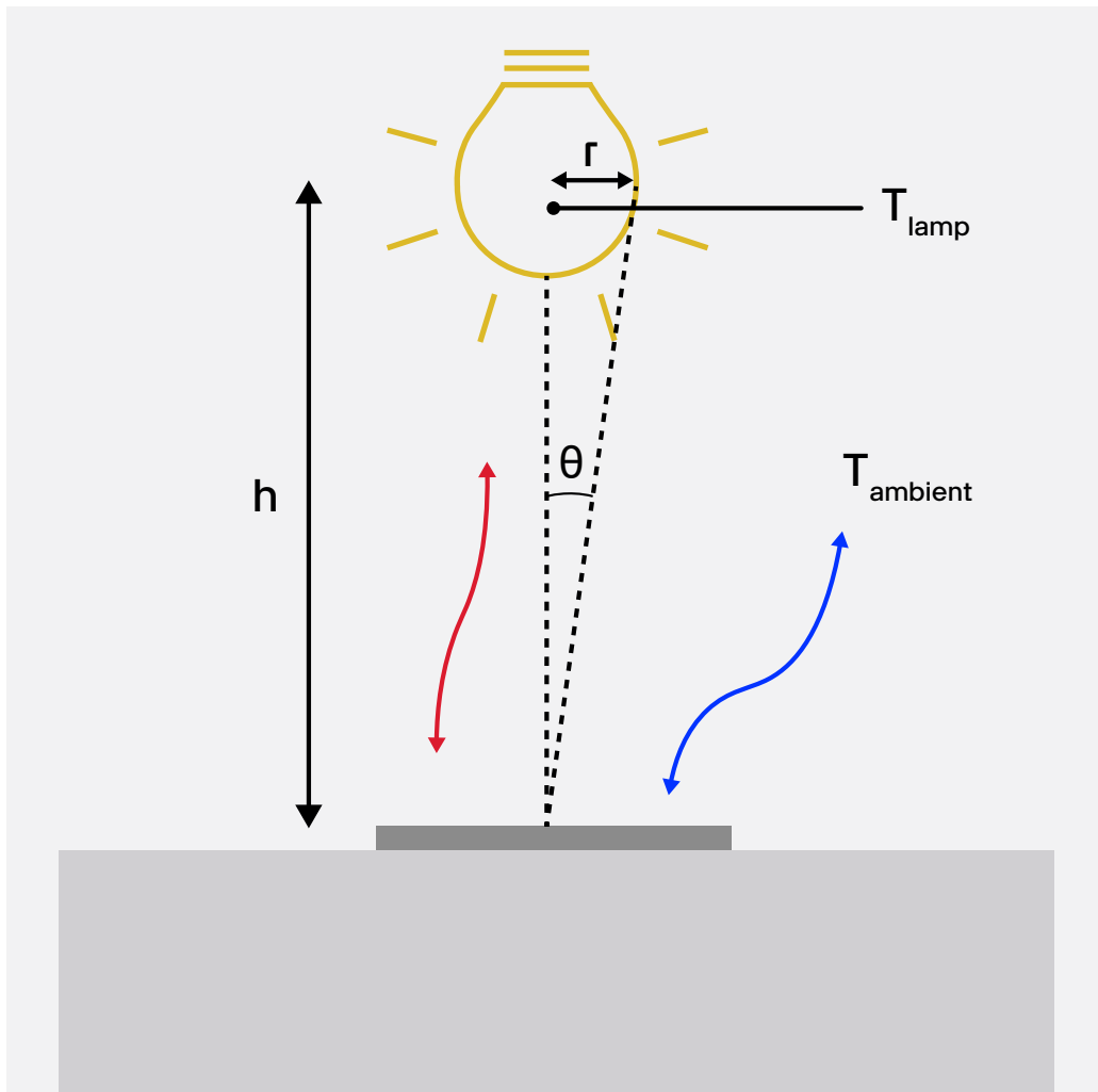
Figure 4.2.1 Measuring radiative heat flux of a round source (as seen from the heat flux sensor). The sensor is situated on a heat sink at T_{\text{sensor}} . The source does not fully occupy the full field of view of the sensors. Radiation from the source originates from an angle \theta .
