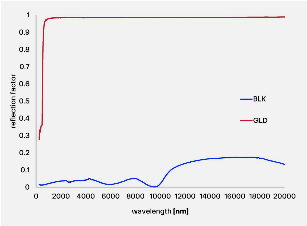
Figure 3.2.11 BLK and GLD reflection factors as a function of wavelength.
