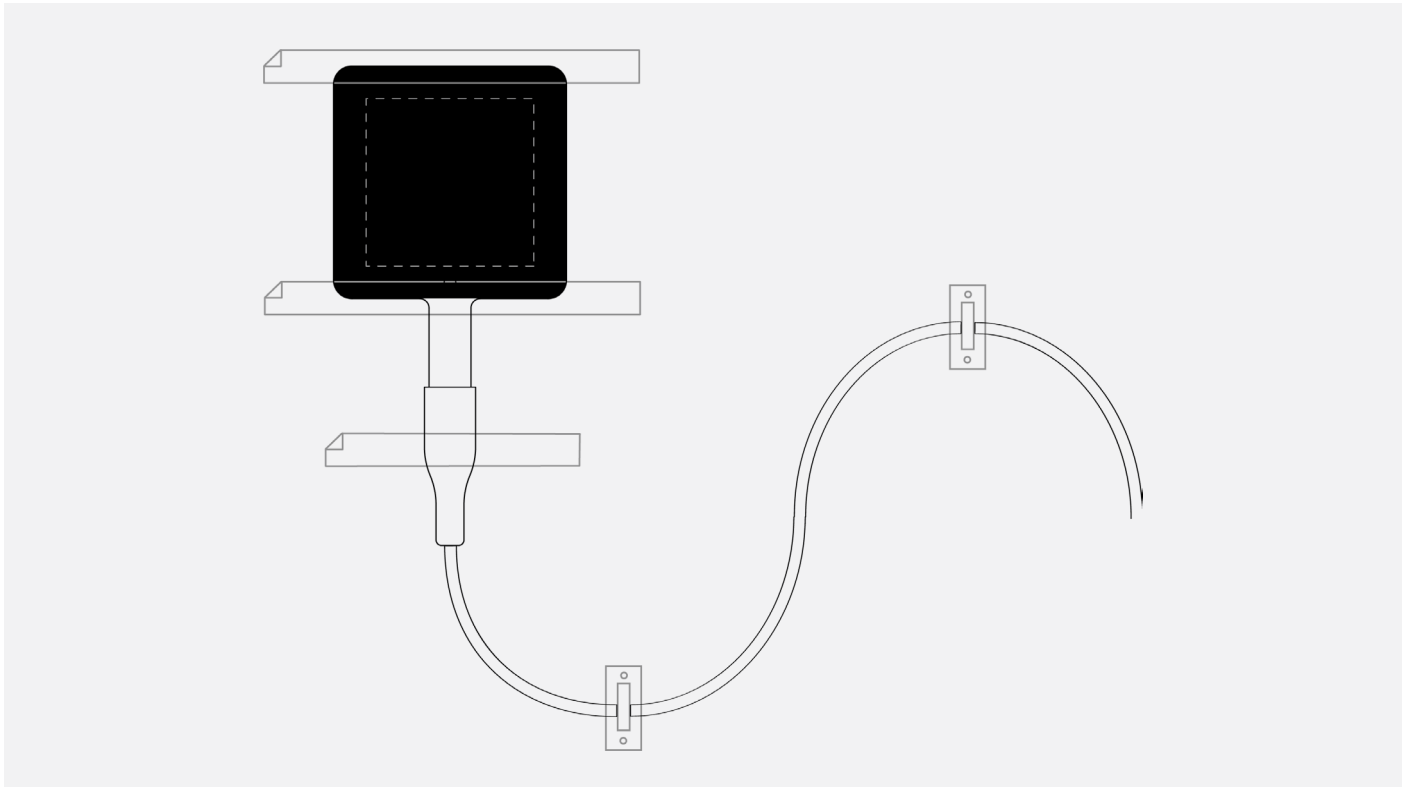
Figure 6.2.1 Installation of model FHF05-50X50 with BLK sticker using tape to attach the sensor and FHF05-50X50 cable connection block serving as strain relief. Extra strain relief on the wires may be provided using cable tie mounts equipped with double-sided adhesive tape. As indicated in the sensor manual, tapes for mounting of the sensor should only cover the passive guard area and not over the sensing area (the latter indicated by a dashed line).
