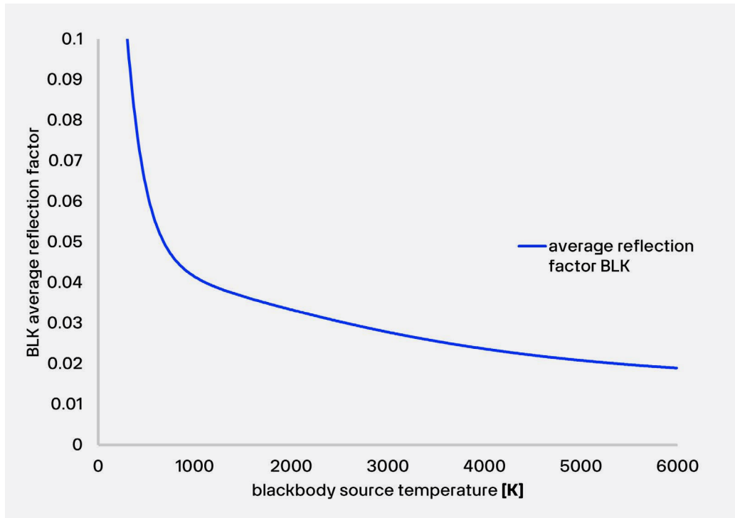
Figure 8.1.3 Average reflection factor of BLK sticker when measuring radiation from blackbody sources of different temperatures.
