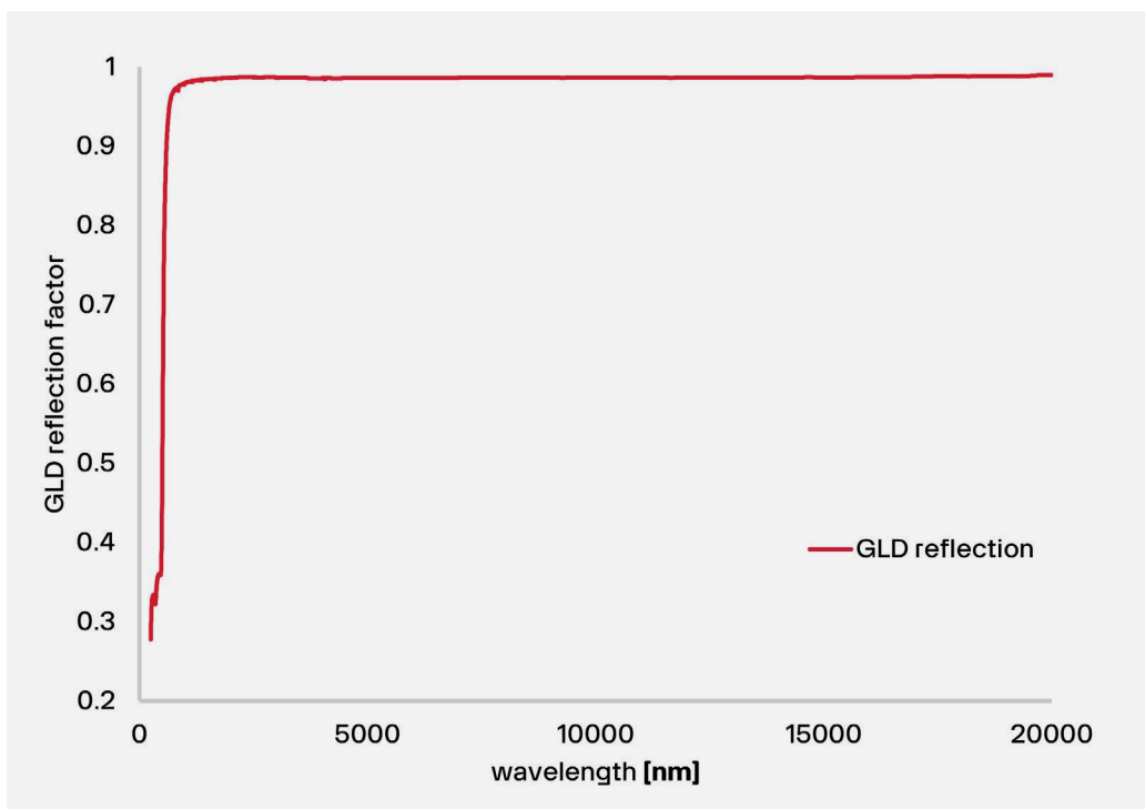
Figure 8.1.2 Reflection factor of GLD sticker as a function of the wavelength of the incoming radiation.
